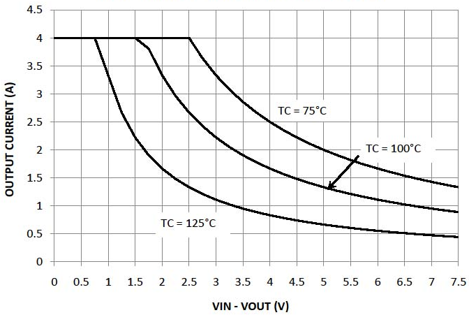
SOA OUTPUT CURRENT vs. VOLTAGE DROP
