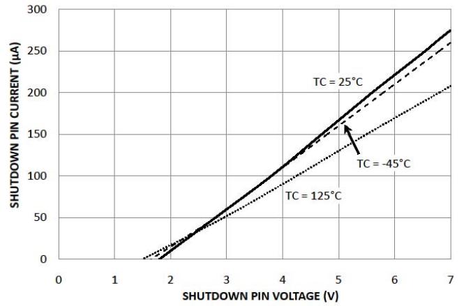
SHUTDOWN PIN CURRENT vs. SHUTDOWN PIN VOLTAGE
