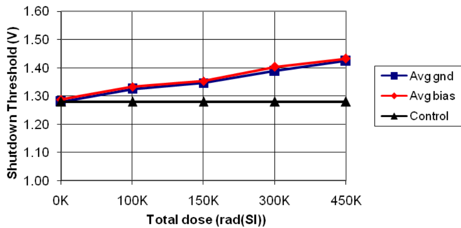
MSK5810KRH Shutdown Threshold vs. Total Dose
