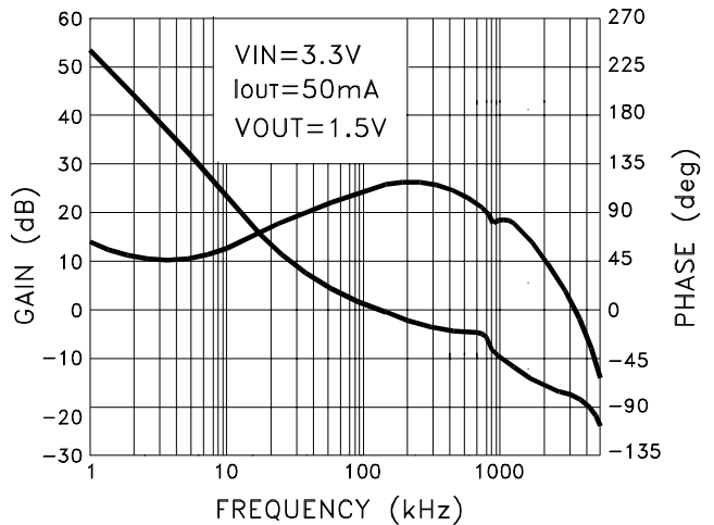
MSK5820RH GAIN AND PHASE vs. FREQUENCY
