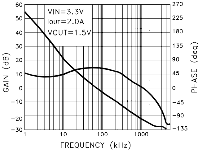
MSK5820RH GAIN AND PHASE vs. FREQUENCY
