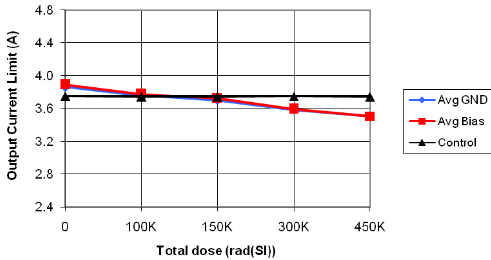
MSK5810KRH Output Current Limit vs. Total Dose
