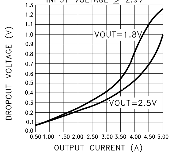
DROPOUT VOLTAGE vs. OUTPUT CURRENT INPUT VOLTAGE ≥ 2.9V
