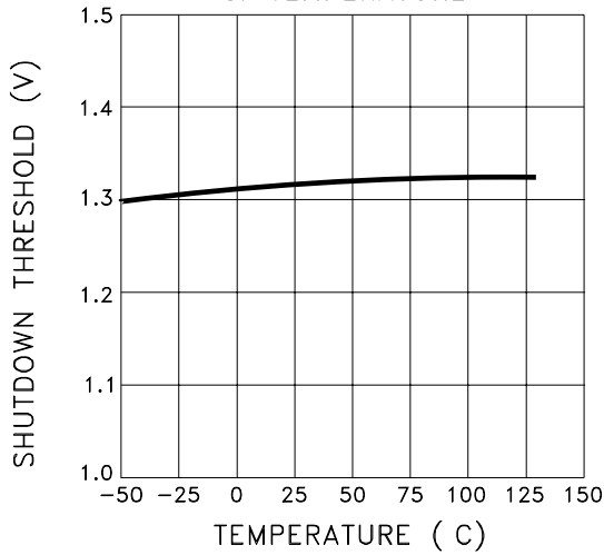
SHUTDOWN VOLTAGE THRESHOLD vs. TEMPERATURE
