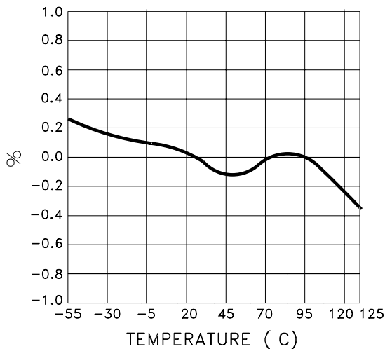
NORMALIZED OUTPUT VOLTAGE vs. TEMPERATURE
