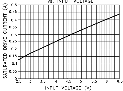
SATURATED DRIVE CURRENT vs. INPUT VOLTAGE
