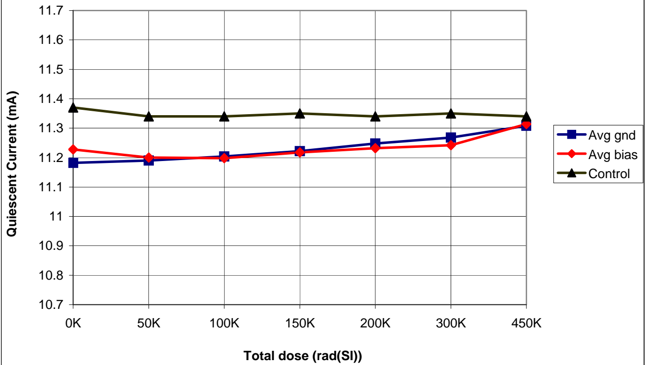
MSK5950RH Quiescent Current vs. Total Dose
