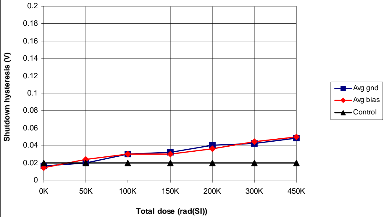
MSK5950RH Shutdown Hysteresis vs. Total Dose
