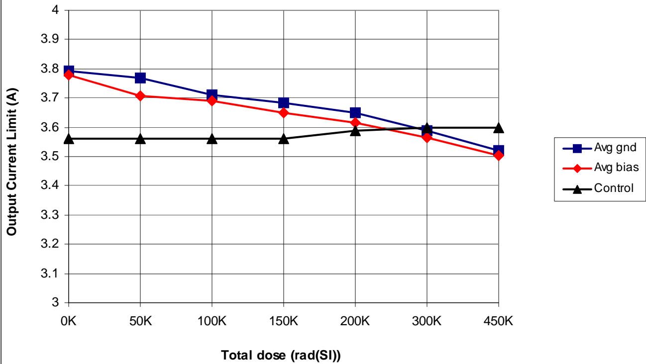
MSK5950RH Output Current Limit vs. Total Dose
