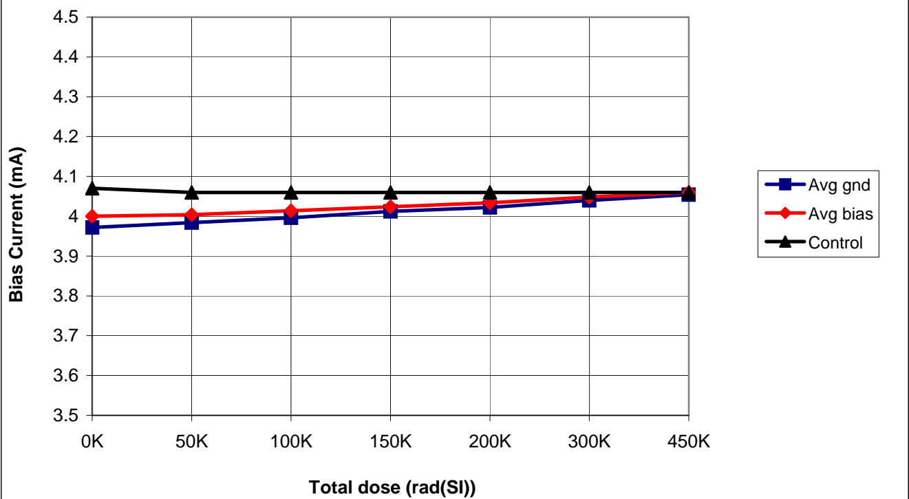
MSK5950RH Bias Current vs. Total Dose
