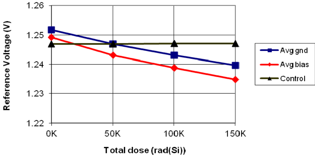
MSK5970RH Reference Voltage vs. Total Dose
