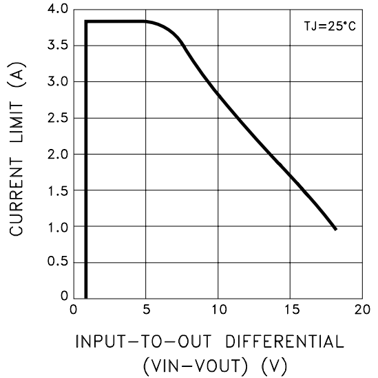
CURRENT LIMIT
