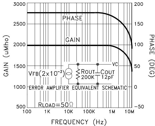
ERROR AMPLIFIER TRANSCONDUCTANCE vs FREQUENCY
