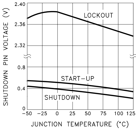
LOCKOUT AND SHUTDOWN THRESHOLDS vs JUNCTION TEMPERATURE
