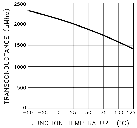
ERROR AMPLIFIER TRANSCONDUCTANCE vs JUNCTION TEMPERATURE
