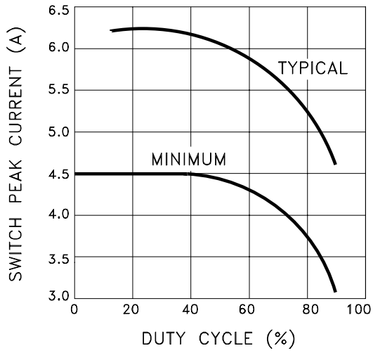
SWITCH PEAK CURRENT LIMIT vs DUTY CYCLE
