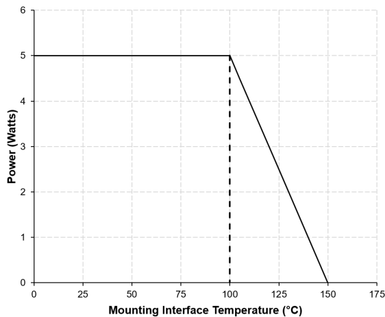
C5A50Z5-F12 Power Derating Curve
