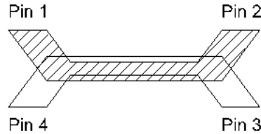
20dB Coupler Pin Configuration
