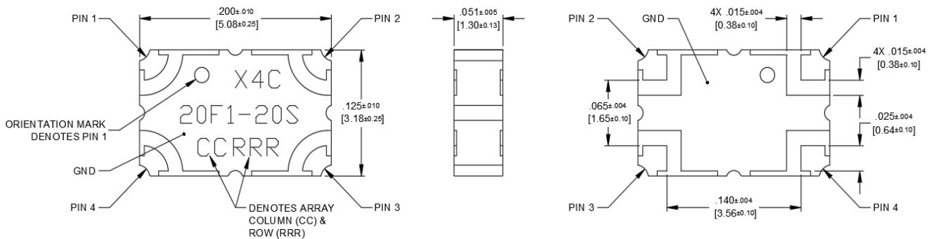
Dimensions are in Inches [Millimeters] X4C20F1-20S Mechanical Outline
