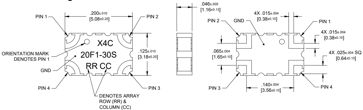
Dimensions are in Inches [Millimeters] X4C20F1-30S Mechanical Outline
