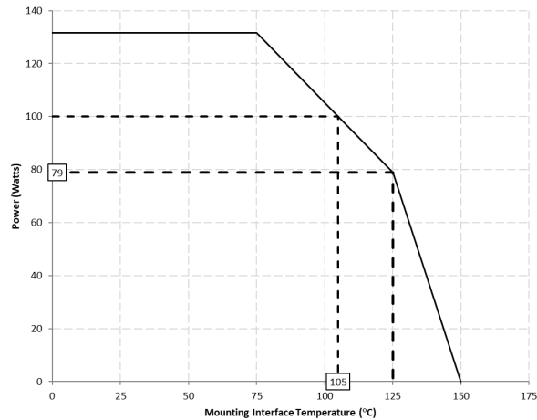
X4C50F1-30S Power Derating Curve
