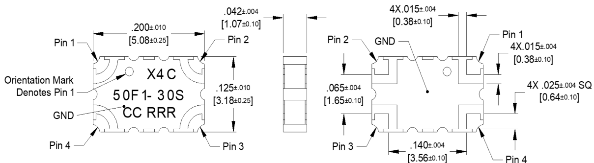
Dimensions are in Inches [Millimeters] X4C50F1-30S Mechanical Outline
