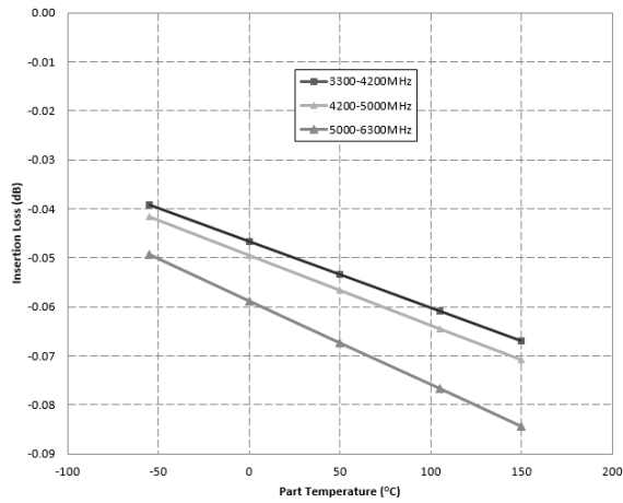
X4C50F1-30S Typical Insertion Loss Derating Curve
