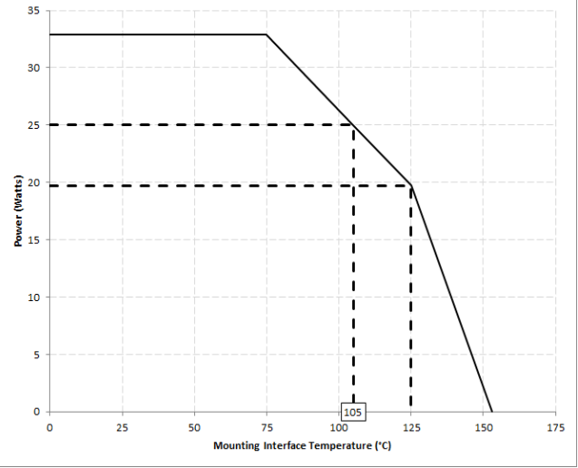
X4C60K1-20S Power Derating Curve
