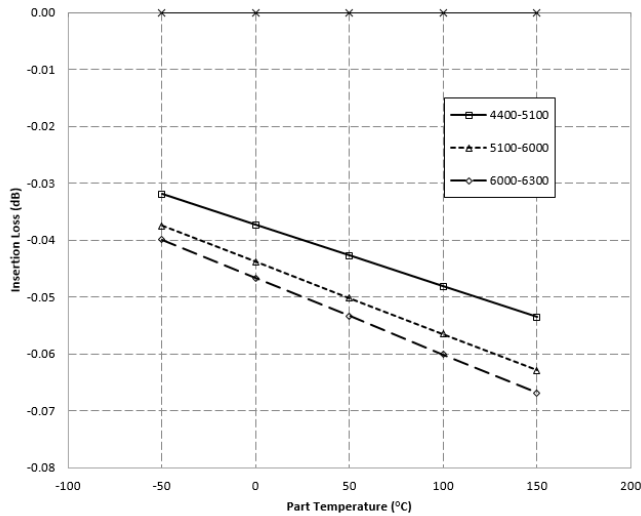
X4C60K1-20S Typical Insertion Loss Derating Curve
