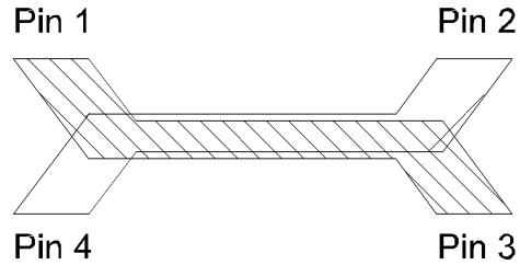
5 dB Coupler Pin Configuration
