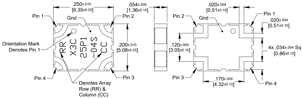
Dimensions are in Inches [Millimeters] X3C25P1-04S Mechanical Outline
