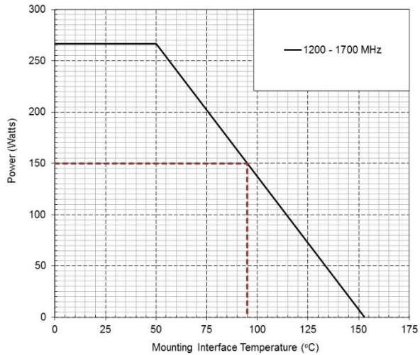
X3C14P1-03S Power Derating Curve 1200-1700 MHz
