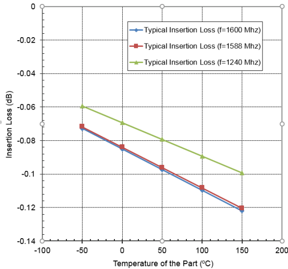
Typical Insertion Loss Derating Curve for X3C14P1-03S
