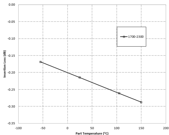
X4C20K1-03S Typical Insertion Loss Derating Curve
