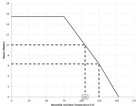
X4C20K1-03S Power Derating Curve
