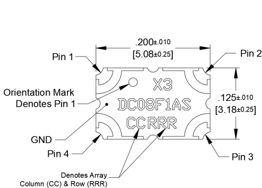
Dimensions are in Inches [Millimeters] X3DC08F1AS Mechanical Outline
