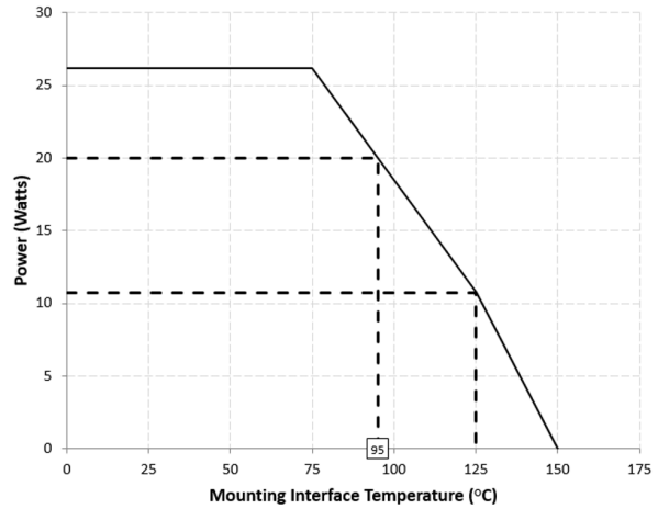
XPS30F190S Power Derating Curve
