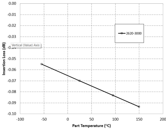
XPS30F190S Typical Insertion Loss Derating Curve
