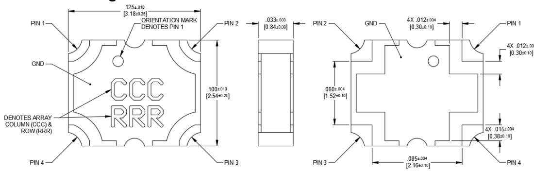
Dimensions are in Inches [Millimeters] X4C20K1-05S Mechanical Outline
