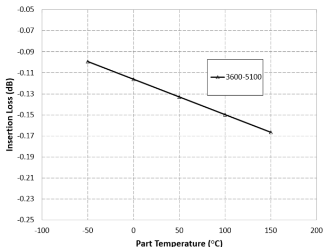
X4C45K1-05S Typical Insertion Loss Derating Curve
