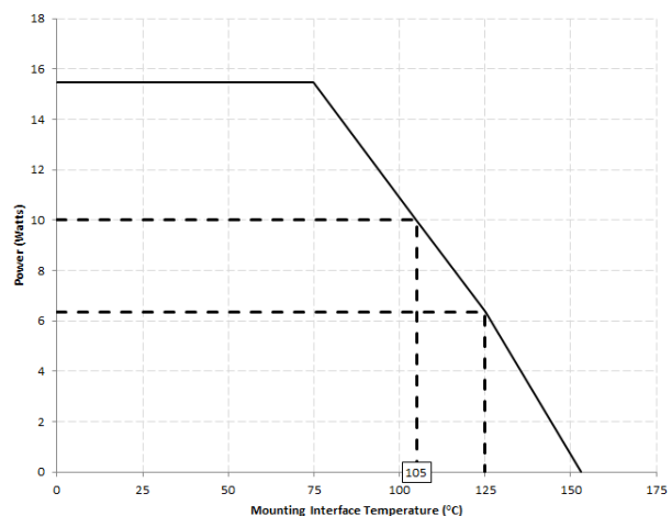
X4C45K1-05S Power Derating Curve
